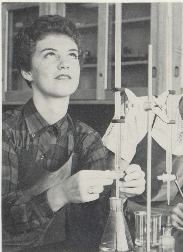
Susie Bolen is performing a chemistry experiment in titration in which the strength of an acid or a base may be determined.
