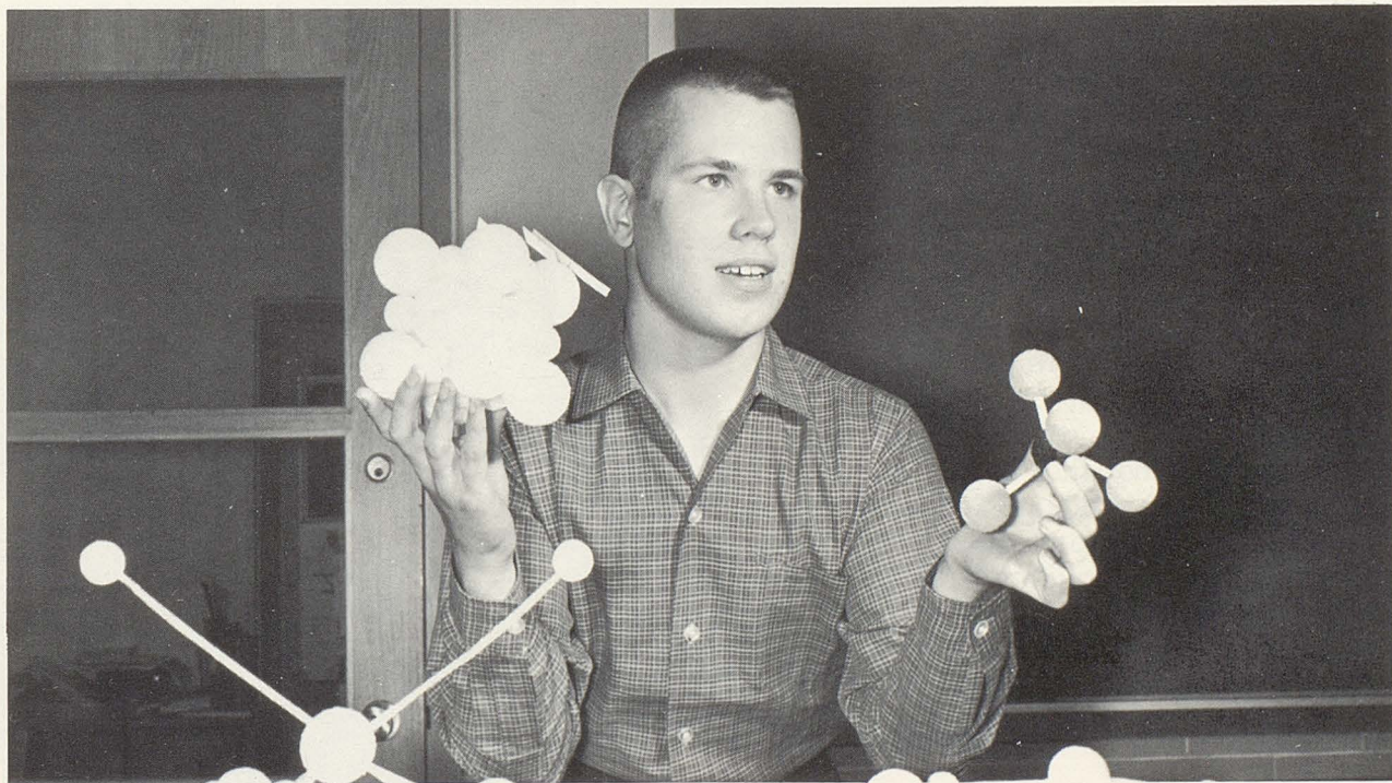
Bob Grosskreutz explains the difference in the electron configuration of two different atoms. His
